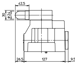
AGIR-20: Mass = 5,5 Kg AGIRR-20: Mass = 5,7 Kg
