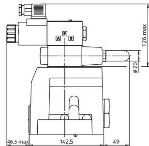
AGIU-32/10/**-E(R)X; Mass = 11,7 Kg
