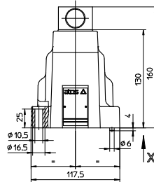
AGIR-32: Mass = 9,4 Kg AGIRR-32: Mass = 9,6 Kg
