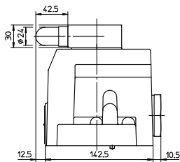
AGIR-32: Mass = 9,4 Kg AGIRR-32: Mass = 9,6 Kg
